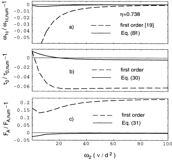
FIG. 2. Comparison of analytic approximations for the coefficients of the stochastic amplitude equation with numerical results for a radius ratio \eta = 0.738 : (a) critical outer rotation \omega_{1c} , (b) time constant \tau_0 , and (c) noise strength F_A of the amplitude equation. Plotted are the relative deviations \delta x = (x_{\text{approx}} - x_{\text{num}})/x_{\text{num}} , where x = \omega_{1c} , \tau_0 , or F_A , for the approximations of this work, Eqs. (B1), (30), and (31), respectively (straight lines), and for the approximations of Ref. [19] (broken lines) as a function of the dimensionless outer rotation \omega_2 .
