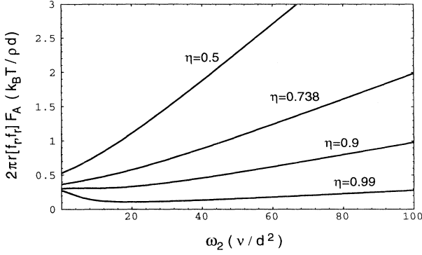
FIG. 3. Cross-section-integrated noise intensity 2\pi r [f_r, f_r] F_A = \int_C d^2 r_\perp |f_r|^2 F_A as a function of \omega_2 with the radius ratio \eta as parameter. The cross-section-integrated fluctuations of the radial velocity in scaled units are (2\sqrt{\epsilon})^{-1} times this quantity.
