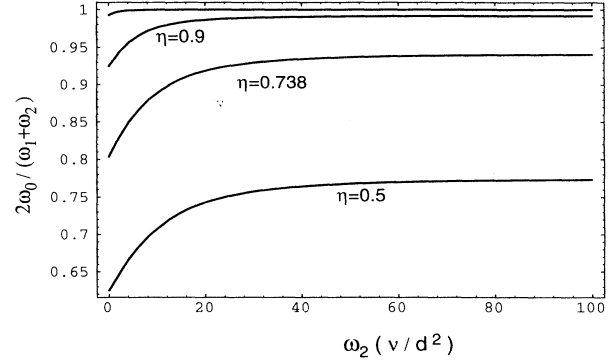
FIG. 1. Ratio of the second-order approximation \omega(r) \approx \omega_0 used in this work and \omega(r) \approx (\omega_1 + \omega_2)/2 used in Ref. [19] as a function of the dimensionless outer rotation \omega_2 = \Omega_2 d^2 / \nu . The parameter is the radius ratio with values \eta = 0.99 (top curve), 0.9 , 0.738 , and 0.5 .
